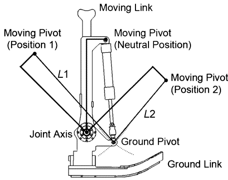
Fig. 16. Solving for the actuator end-point. First, an actuator and moving pivot location (in the neutral position) were chosen. The actuator is fully extended (length L_1 ) and fully contracted (length L_2 ) at the limits of motion (positions 1 and 2). The second end-point, the ground pivot, is found by the intersection of arcs of radii L_1 and L_2 centered at the moving pivot positions 1 and 2.
