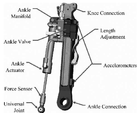
Fig. 23. BLEEX shank design.
