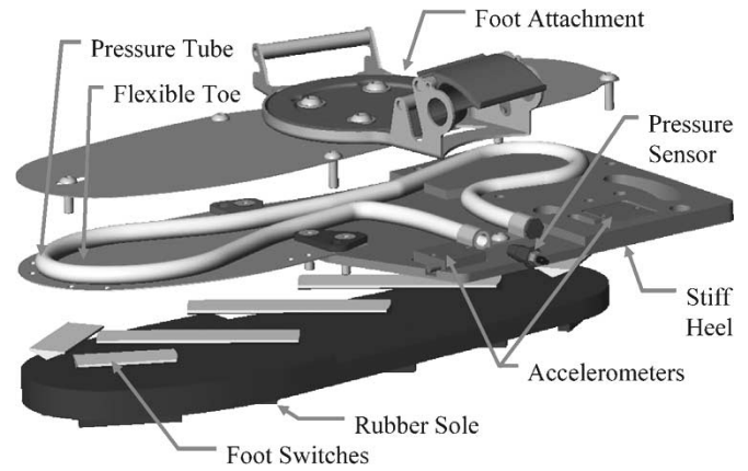
Fig. 22. BLEEX foot design (exploded view).
